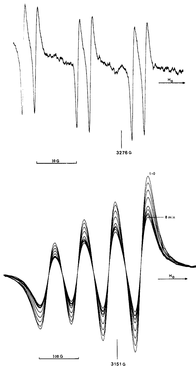
Figure 1. ESR spectra of the benzophenone-sensitized photoreduction of Cu(acac) 2 in the presence of 2-nitroso-2-methylpropane. (a, top) Two-minute irradiation of a methylene chloride solution of Cu(acac) 2 (1 mM), NMP (2 mM), and benzophenone (5 mM): a_N = 13.62 , a_H = 3.15 G, g value 2.0062. (b, bottom) Irradiation of the same solution with the monitor of the Cu(acac) 2 signal at every minute.
